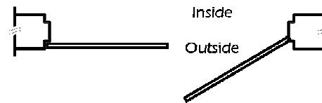
Right Hand Reverse Active (RHRA)
